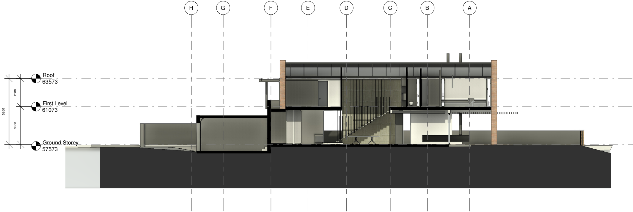
1 DC A3000 (Section) 1-1 1 : 200
