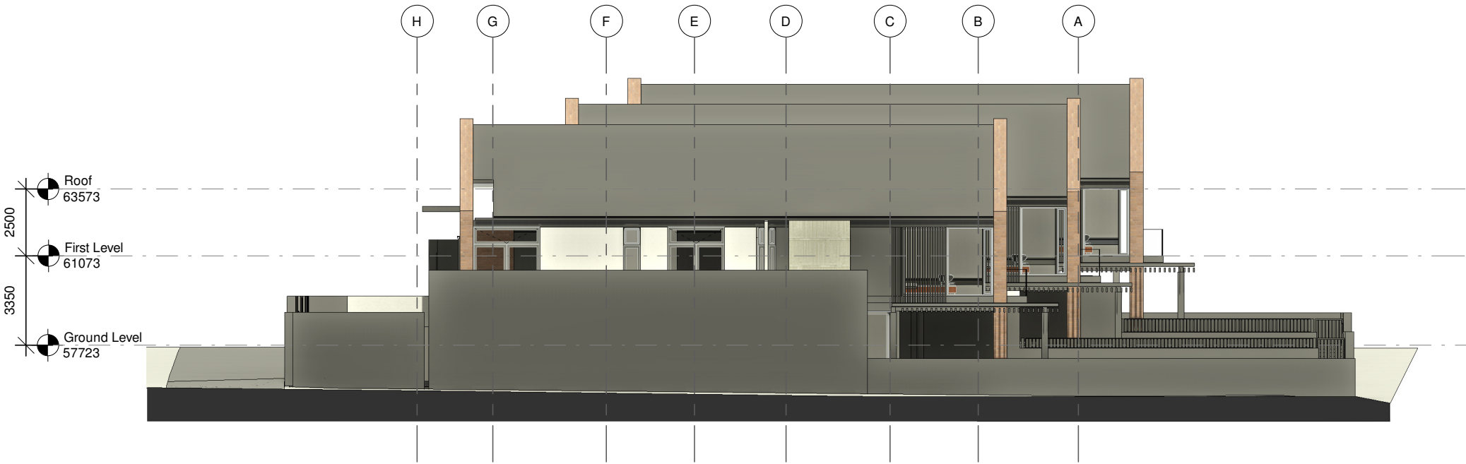
1 DC A2000 (Elevation) 03 East 1 : 200
